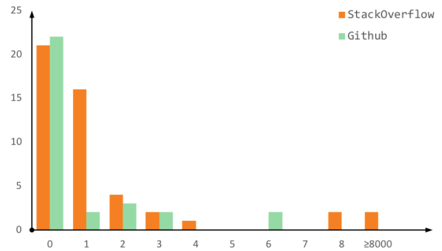
Figure 8: Dependency Distance Distribution
